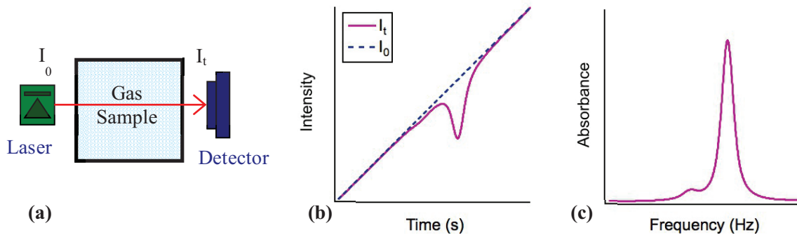
Fig. 1-2. Example tunable diode laser absorption spectroscopy measurement. (a) A schematic of laser light at a known frequency passing through a gas sample of interest. (b) A sample intensity/wavelength sweep of the laser demonstrating the attenuation of the incident light ( I_0 ) by absorption by the gas sample to result in the transmitted ( I_t ) light intensity. (c) Absorbance as a function of frequency calculated from b) using the Beer-Lambert law and a measured frequency sweep.
