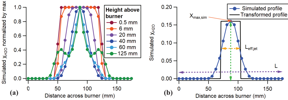
Fig. 4-2 (a). Extracted H 2 O mole fraction profiles across the width of the catalytic combustor from the CFD simulation of the heated, buoyant jet above the catalytic surface. (b) Simulated H 2 O mole fraction profile as a function of distance across the burner at 18 mm above the surface and the corresponding top-hat profile with the same area, and a height of \chi_{\max, \text{sim}} and a width of L_{\text{eff, jet}} calculated using Eq. (4).
