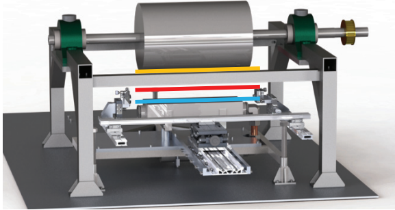
Fig. 4-14. Experimental set up of varying equivalence ratio with chilled roller characterization of heated buoyant jet with a gap of 0.375 inches. The yellow line indicates the laser beam passing through the jet right at the surface of the roller, the red indicates the midline measurement (.25”) and the blue indicates the beam passing the combustor surface.
