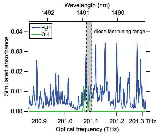
Fig. 2-1. Simulated absorbance of 15% H 2 O and 0.3% OH mole fraction from 200.9-201.4THz (1489-1493 nm) using HITEMP 2010 for OH and the spectral database developed in this paper for H 2 O. Both species were simulated at 2200 K, 820 mbar, and a pathlength of 30.7 cm. Shaded region indicates tuning range of DFB diode laser used for WMS measurements. The range of the dual – frequency comb spectrometer extends beyond the edge of the plot from 196.2-217.2 THz (1380-1528 nm).
