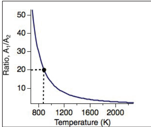
Fig. 1-3. Ratio of linestrengths, S(T) or integrated absorbance, A , for two different H_2O absorption transitions. The ratio of these two quantities is only dependent on temperature, thus enables calculation of temperature.
