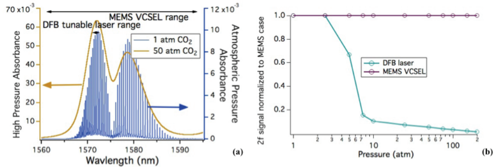
Fig. 5-1. (a) Room temperature absorbance spectrum of carbon dioxide (CO 2 ) at 1 atm and 50 atm, with the corresponding fast-scanning ranges of a traditional DFB diode laser and a MEMS-VCSEL laser (5% CO 2 in air, 100 cm path length). (b) Simulated 2f peak signal for CO 2 using a DFB and the MEMS-VCSEL laser centered around 1570 nm, normalized to the MEMS case, at a series of pressures. As pressure rises above a few atmospheres the DFB laser can no longer reach the optimal modulation amplitude for the broadening absorption conditions.
